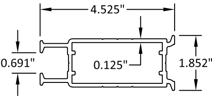
5 1/4" ANCHOR SLEEVE E9-7042
