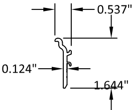
SSG SETTING BLOCK CHAIR (1 5/16" GLASS) E1-7011
