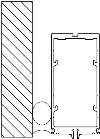
UNREINFORCED JAMB
