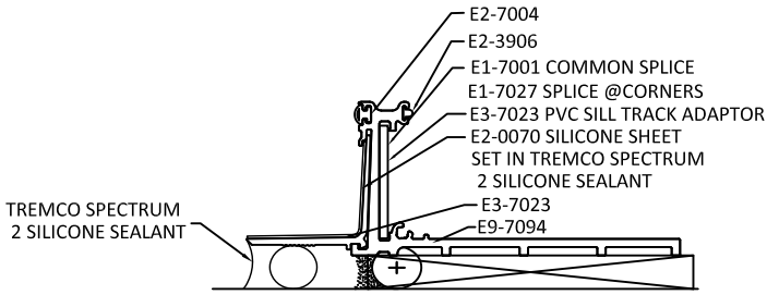
SPLICE & SEALING DETAILS SILL STARTER
