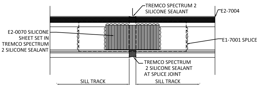
SPLICE & SEALING DETAILS SILL STARTER
