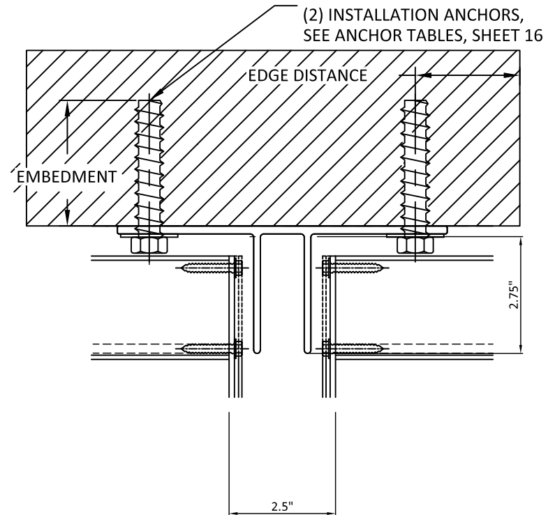
FRONT VIEW T-CLIP AT VERTICAL MULLION HEAD
