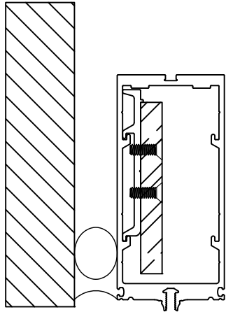
REINFORCED JAMB
