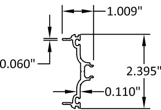
PRESSURE PLATE (1-5/16" GLASS) AS-7057
