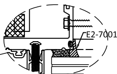
L1 6 HORIZONTAL SECTION REINF. JAMB - E.T.A. WITHOUT ADAPTOR
