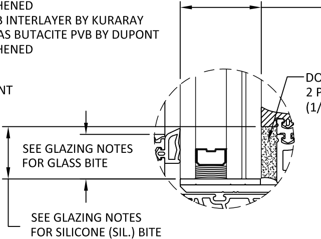
GLAZING OPTION B
