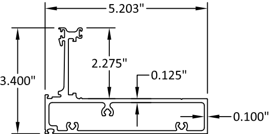
5 1/4" HEAD/HORIZONTAL E9-7027
