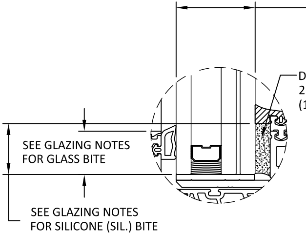
GLAZING OPTION A
