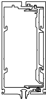
INTERMEDIATE UNREINFORCED VERTICAL
