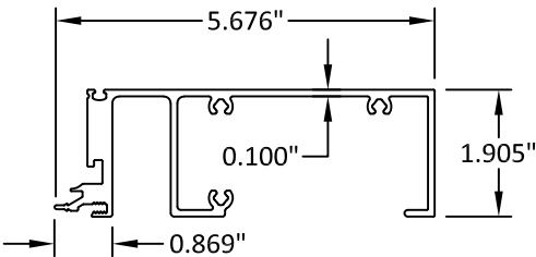
5 1/4" SSG SILL/HORIZONTAL E9-7023
