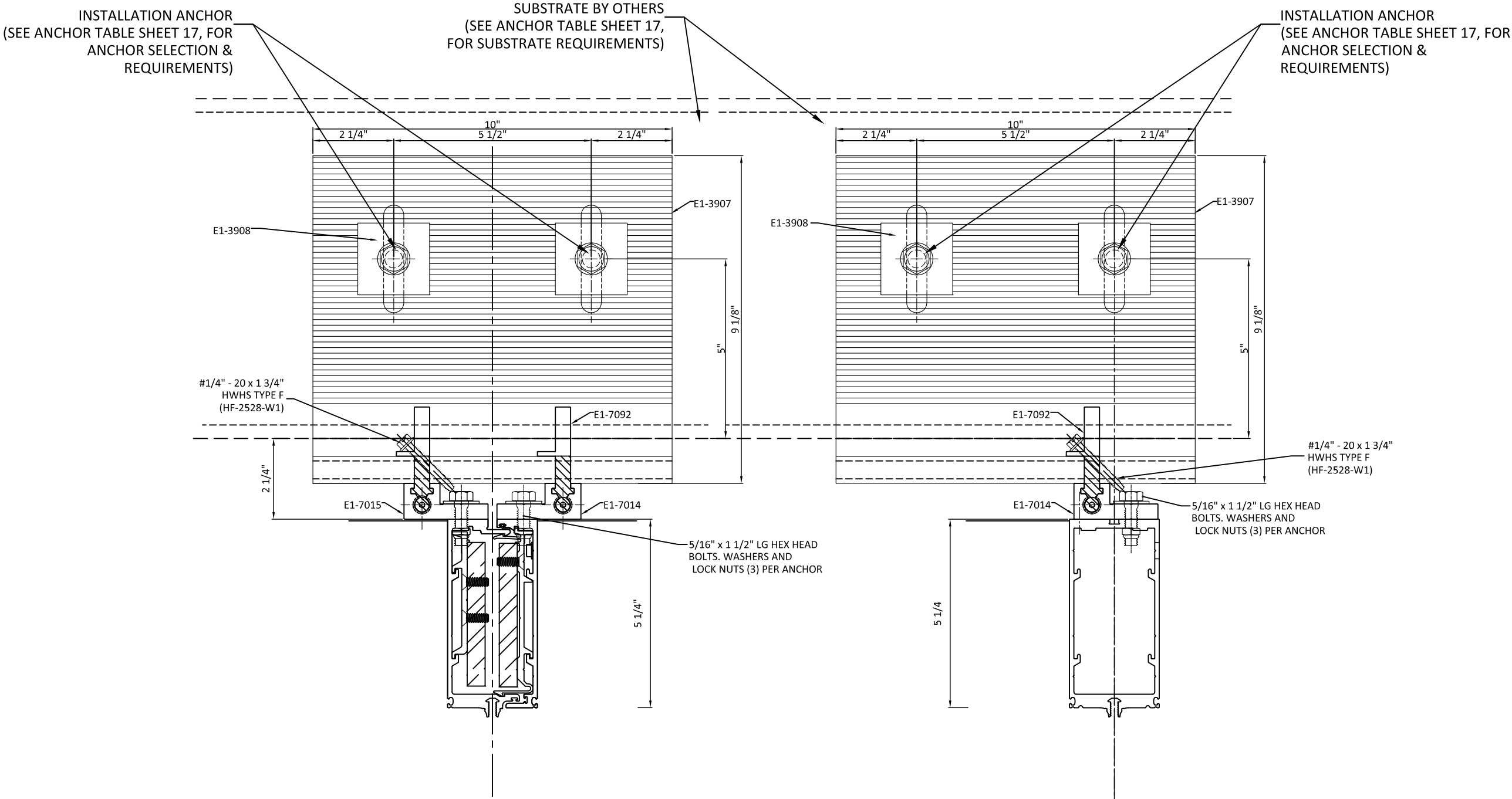
X HORIZONTAL SECTION 18 DEAD LOAD L-ANCHOR INTERMEDIATE VERTICAL MULLION
