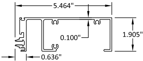
5 1/4" SILL/HORIZONTAL E9-7096
